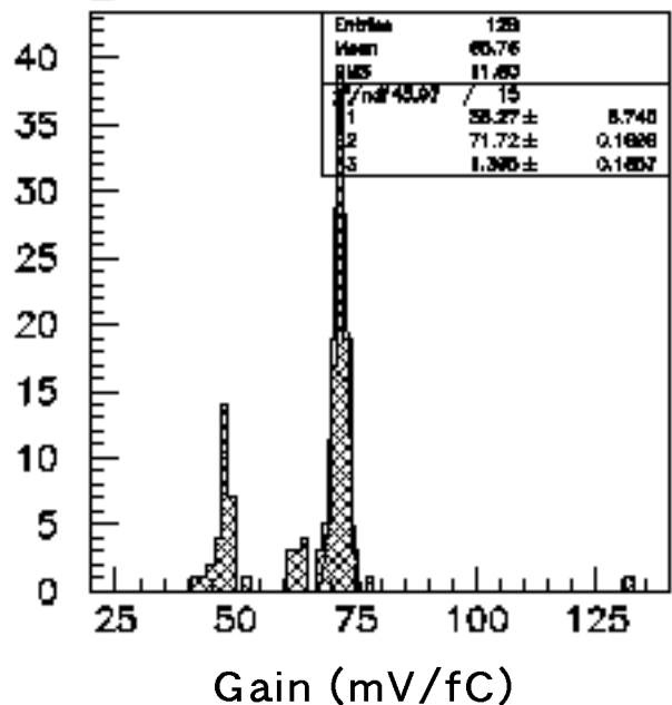
gain distribution
