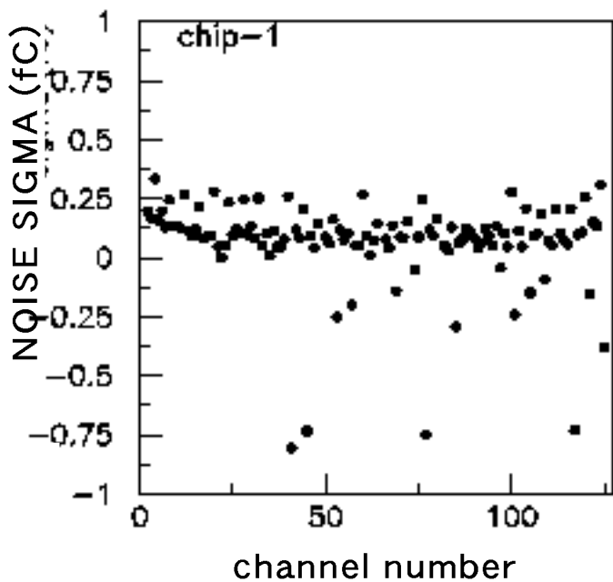
noise vs ch number
