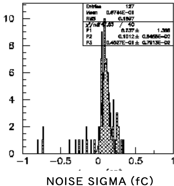
noise distribution
